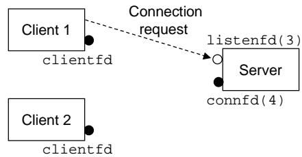
Figure 12.1: Step 1: Server accepts connection request from client.
