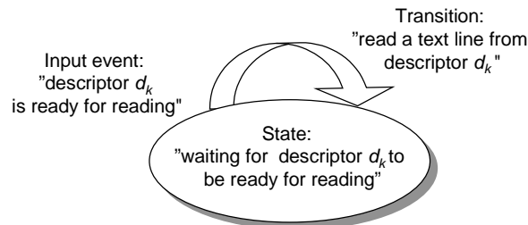
Figure 12.7: State machine for a logical flow in a concurrent event-driven echo server.
