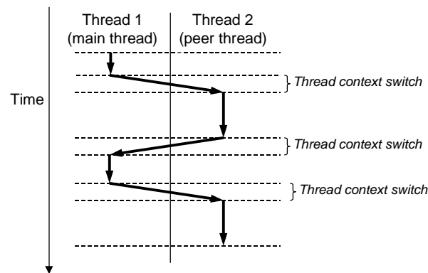
Figure 12.12: Concurrent thread execution.
