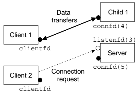
Figure 12.3: Step 3: Server accepts another connection request.
