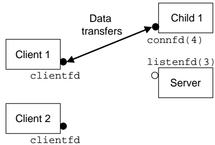
Figure 12.2: Step 2: Server forks a child process to service the client.
